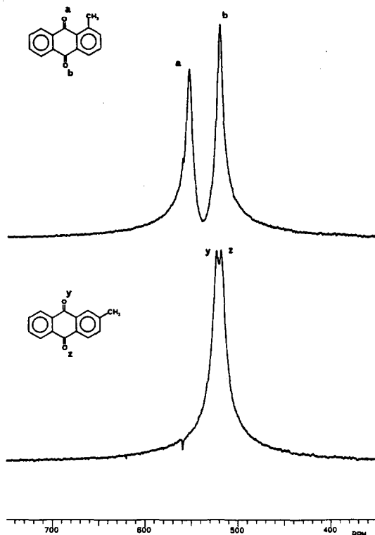
Figure 1. ^{17}\text{O} NMR spectra for 1- and 2-methylanthraquinone:
