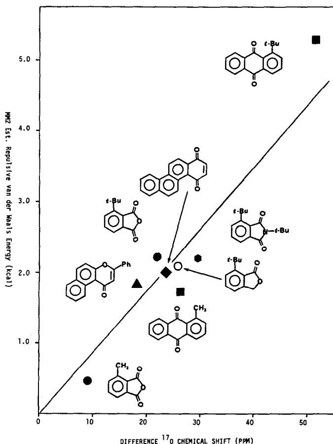
Figure 2. Correlation of est. van der Waals repulsive interactions vs ^{17}\text{O} chemical shift difference values.
